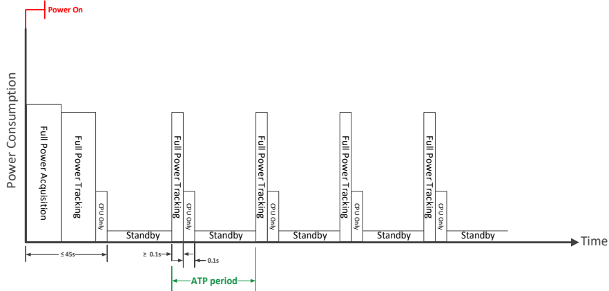
FIGURE 3 – ATP™ TIMING
