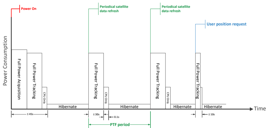
FIGURE 4 – PTF™ TIMING
