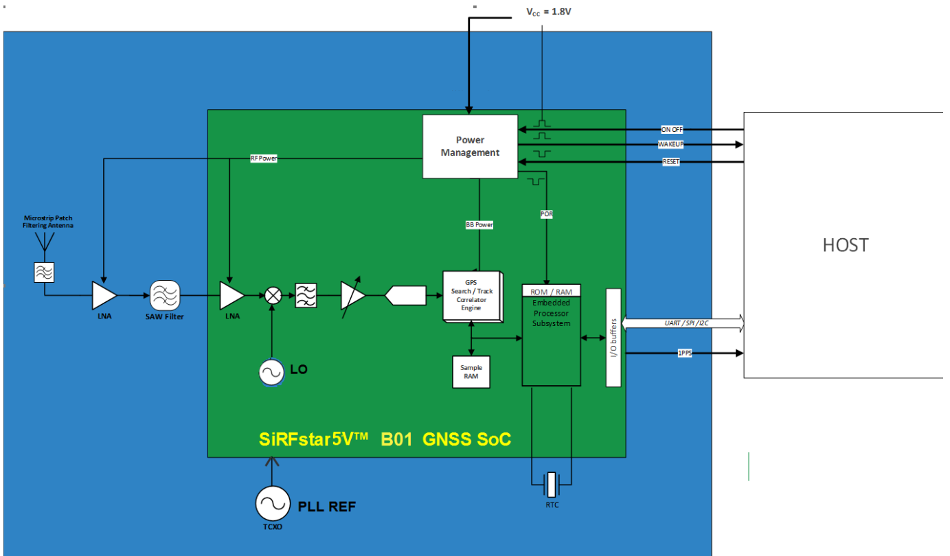
FIGURE 1 – ORG1510 ARCHITECTURE
