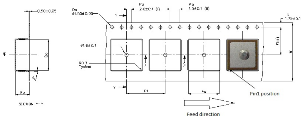
FIGURE 13 – CARRIER TAPE
