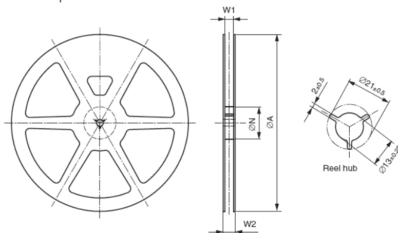
FIGURE 14 – REEL
