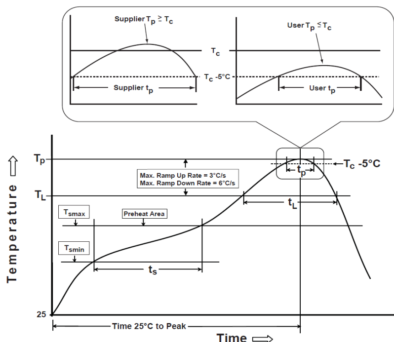
FIGURE 10 – RECOMMENDED SOLDERING PROFILE
