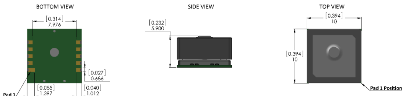
FIGURE 11 – MECHANICAL DRAWING
