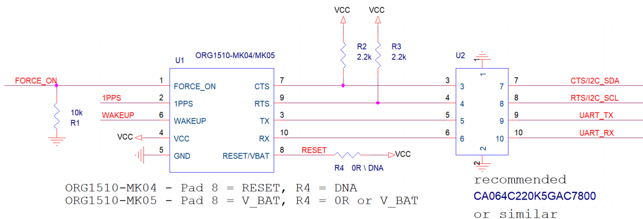
Figure 9. Reference Schematic Diagram
