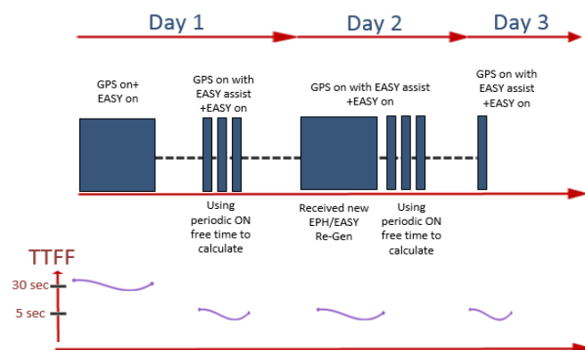
Figure 3. EASY™ TTFF Timing
