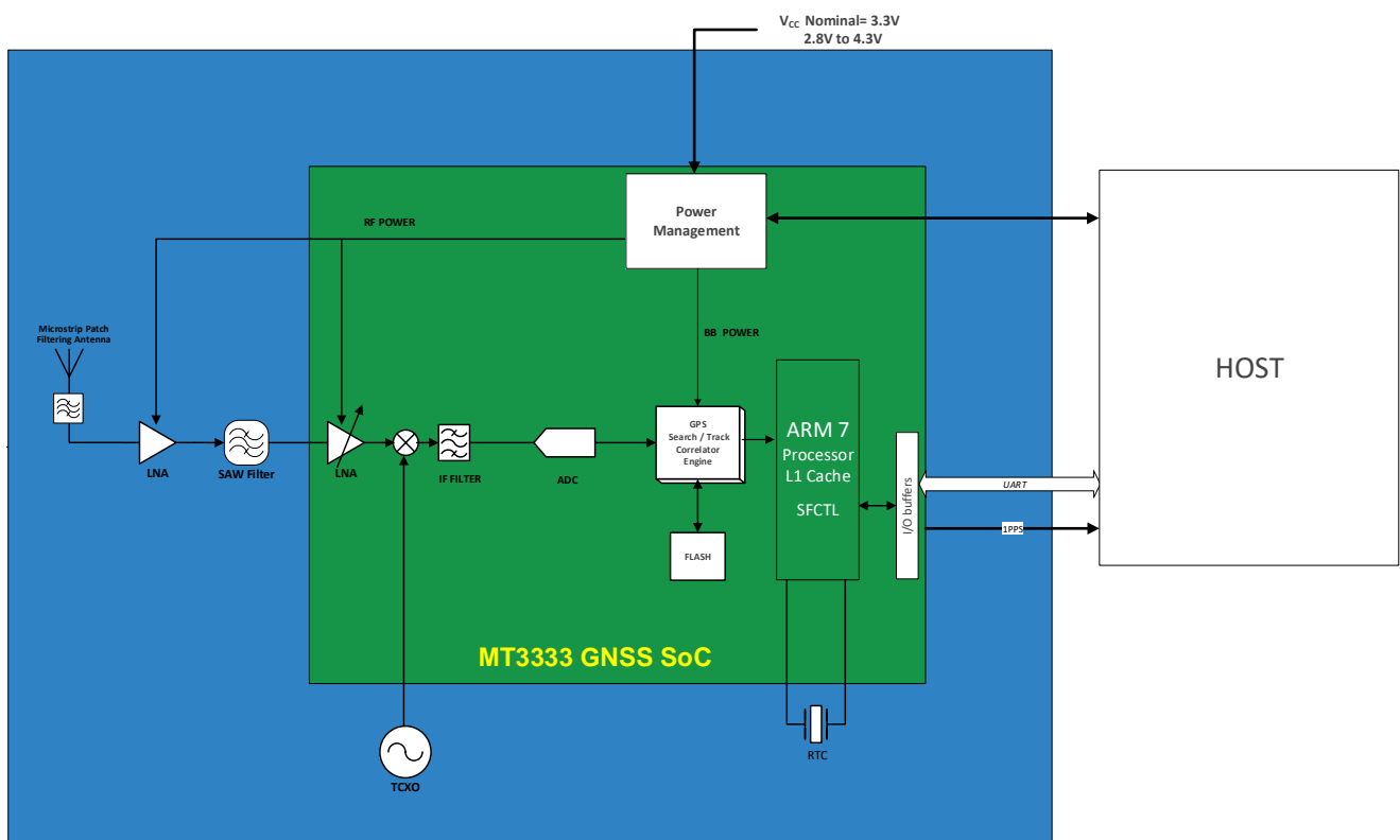
Figure 1. ORG1510-MK04/5 Architecture
