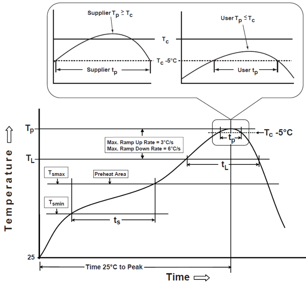
Figure 10. Recommended Soldering Profile
