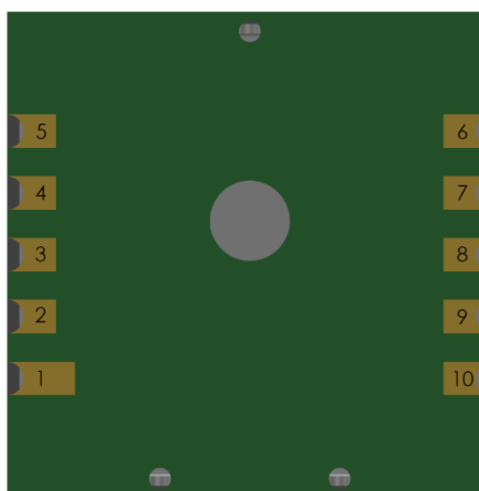
Figure 6. Pads Assignment
