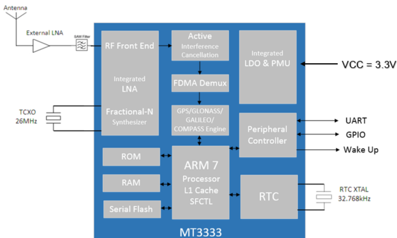
Figure 2. MT3333 System Block Diagram and Peripheral
