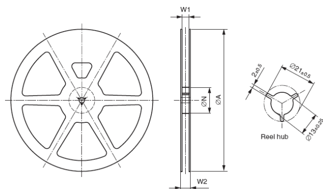
Figure 13. Reel
