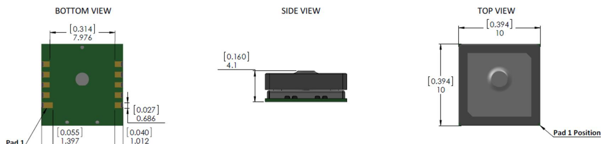
Figure 7. Mechanical Drawing
