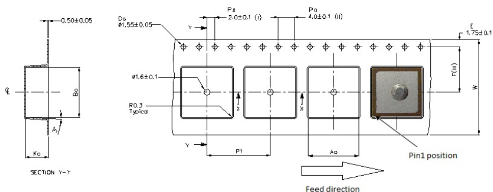
Figure 13. Carrier Tape
