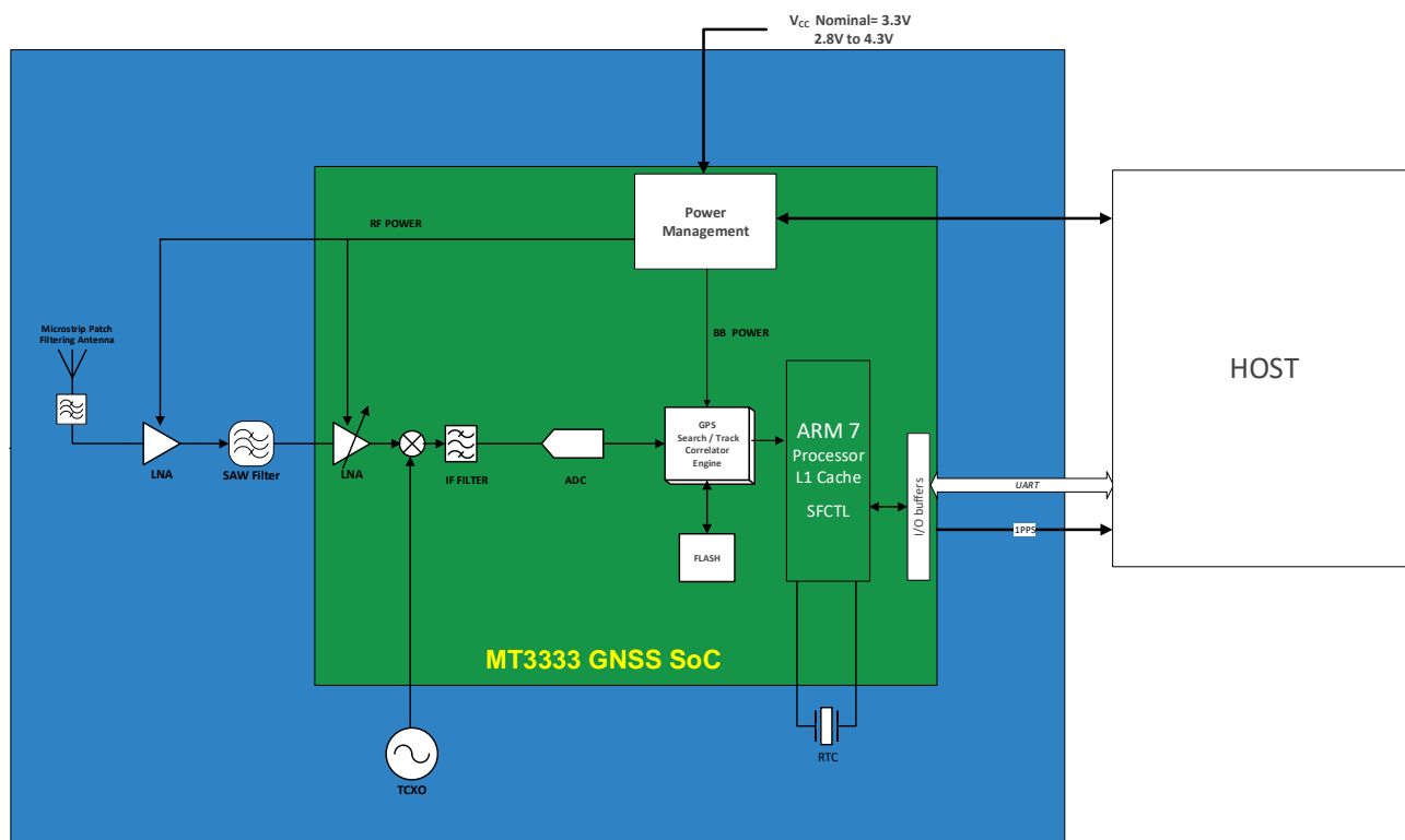
Figure 1. ORG1511-MK05 Architecture
